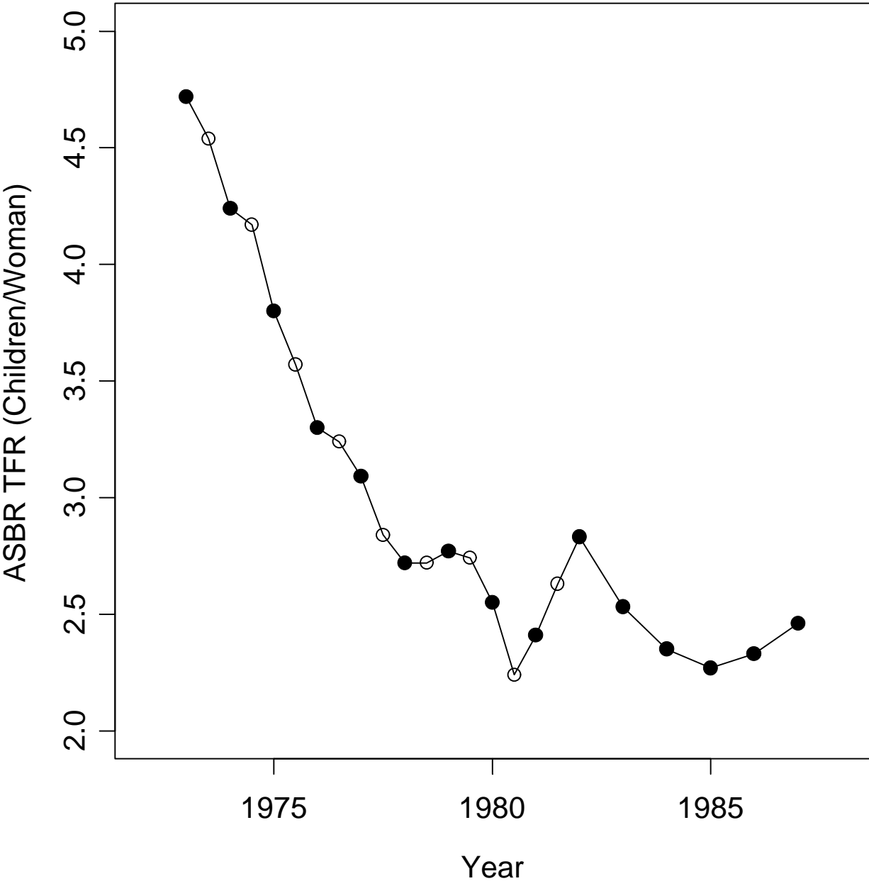
Figure 1 China Age-Specific Birth Rate TFRs
